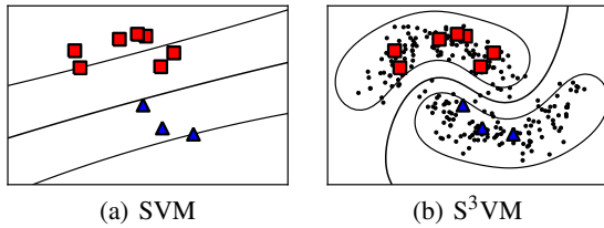
Figure 1: The concepts of support vector machines and their extension to semi-supervised learning settings. Labeled patterns are depicted as red squares and blue triangles and unlabeled patterns as black points, respectively.
