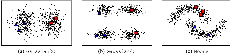
Figure 3: Distribution of all artificial data sets ( d = 2 ). The red squares and blue triangles depict the labeled part of the data; the remaining black points correspond to the unlabeled part. Note that the two Gaussian data sets depict easy learning instances for d = 2 , even given only few labeled patterns. However, the noise present in the data render the induced tasks difficult to approach in high dimensions ( d = 500 ) in case only few labeled patterns are given (for supervised models).
