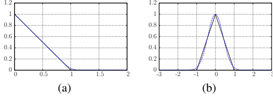
Figure 2: The hinge loss \mathcal{L}(y, t) = \max(0, 1 - yt) and its differentiable surrogate \mathcal{L}(y, t) = \frac{1}{\gamma} \log(1 + \exp(\gamma(1 - yt))) with y = +1 and \gamma = 20 are shown in Figure (a). The effective hinge loss function \mathcal{L}(t) = \max(0, 1 - |t|) along with its differentiable surrogate \mathcal{L}(t) = \exp(-st^2) with s = 3 are shown in Figure (b).
